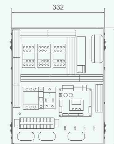
Front Size Dimension
